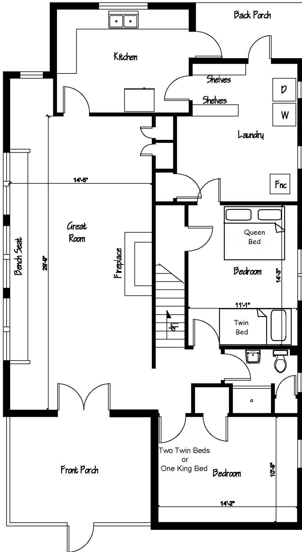
River Lodge 1st Floor Plan
